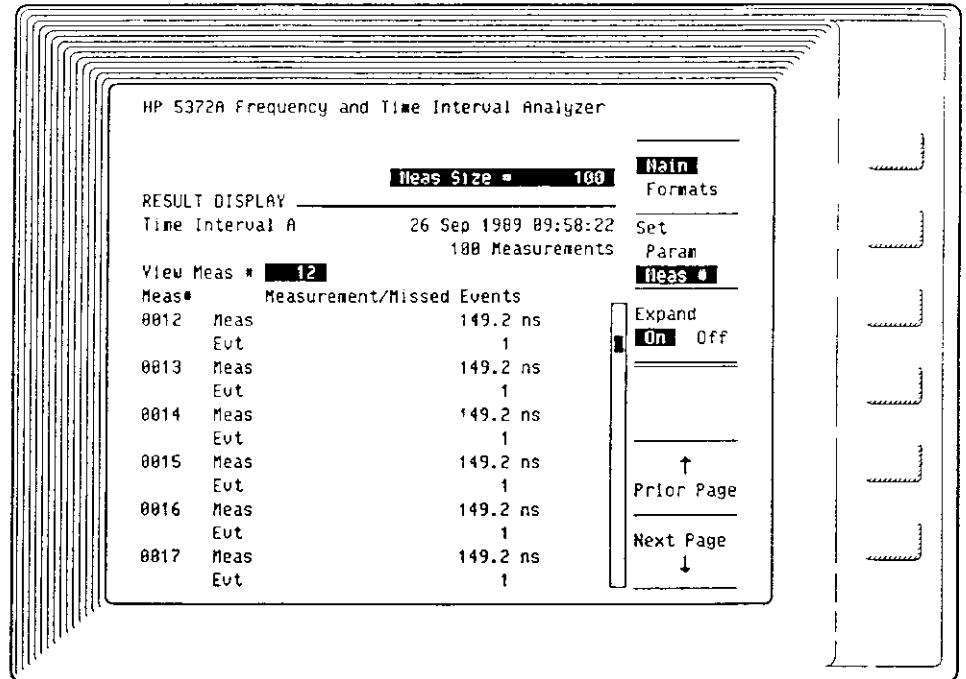
Figure 1-10. Time Interval results
