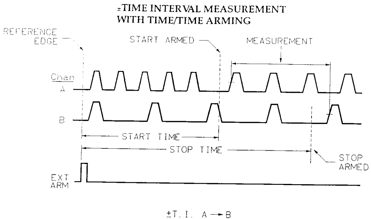
Figure 1-43. ±Time Interval | Time/Time
