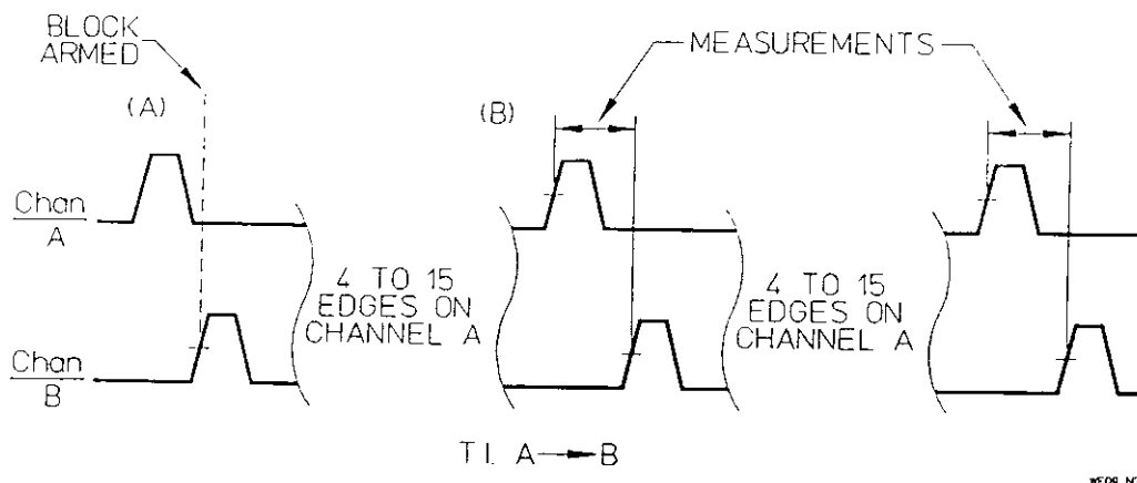
Figure 5-46. EDGE/RANDOM Timing Diagram
