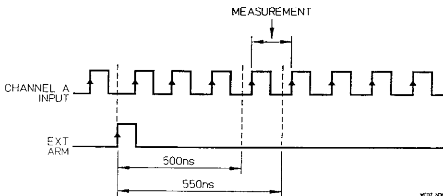
Figure 5-8. More Non-continuous Arming Phrases
