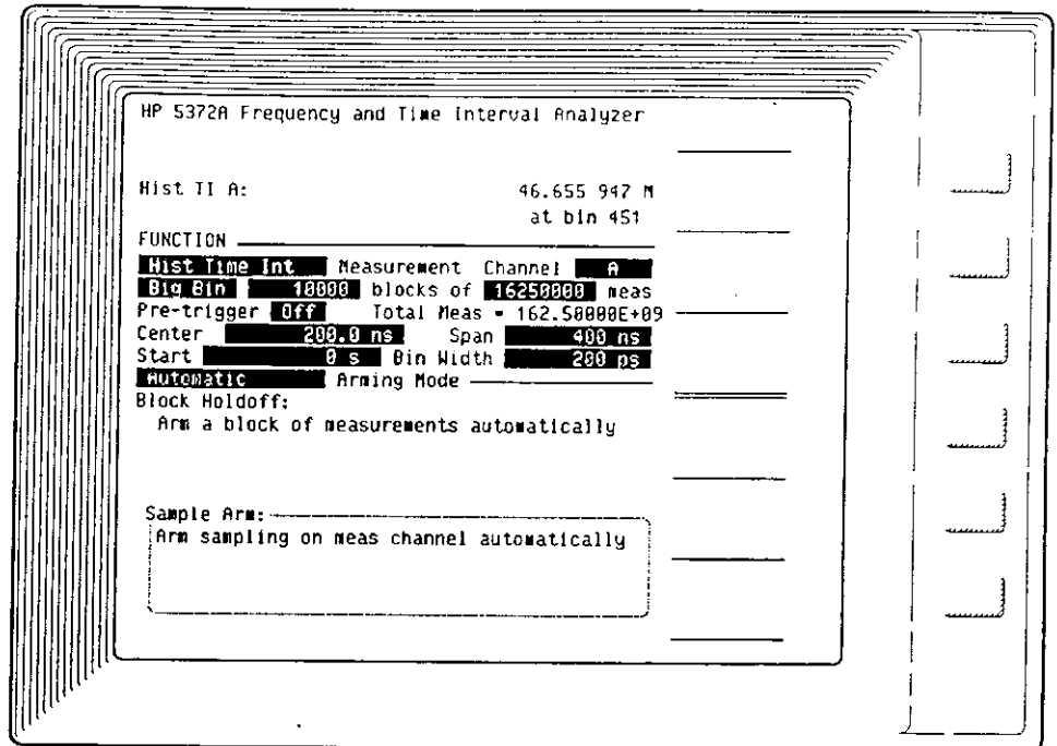
Figure 4-5. Function Menu Configuration To Avoid Bin Overflow
