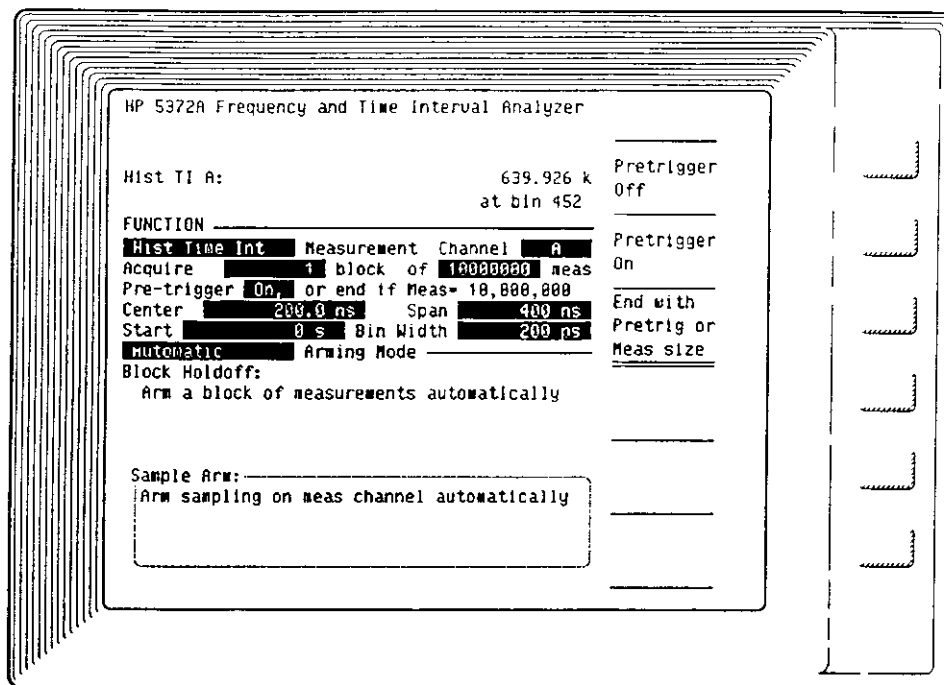
Figure 4-12. Setup 7: One Block — Measurements End on Pre-trigger or Measurements.
