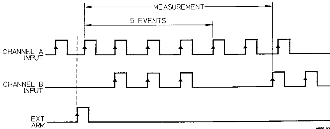
Figure 5-7. Non-continuous Arming Phrases
