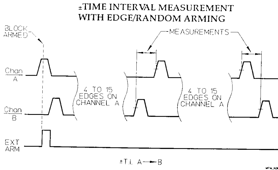
Figure 1-45. ±Time Interval | Edge/Random
