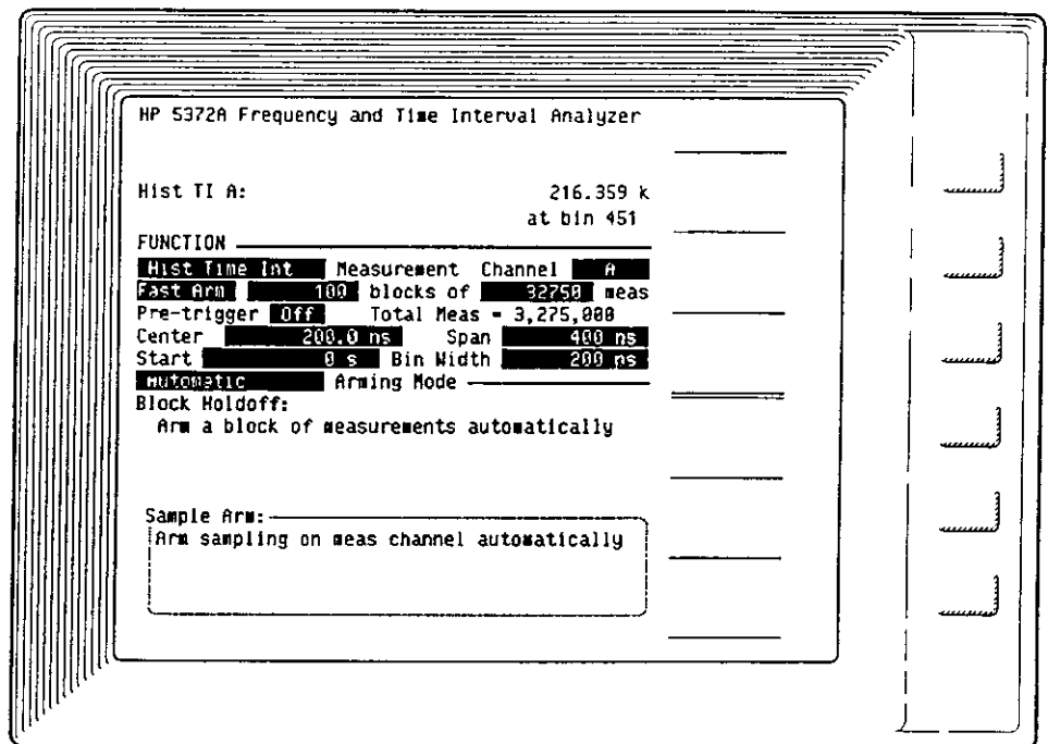
Figure 4-7. Setup 2: M Blocks — Fast Arm Between Blocks
