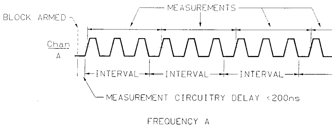
Figure 2-10. Frequency | Interval Sampling
