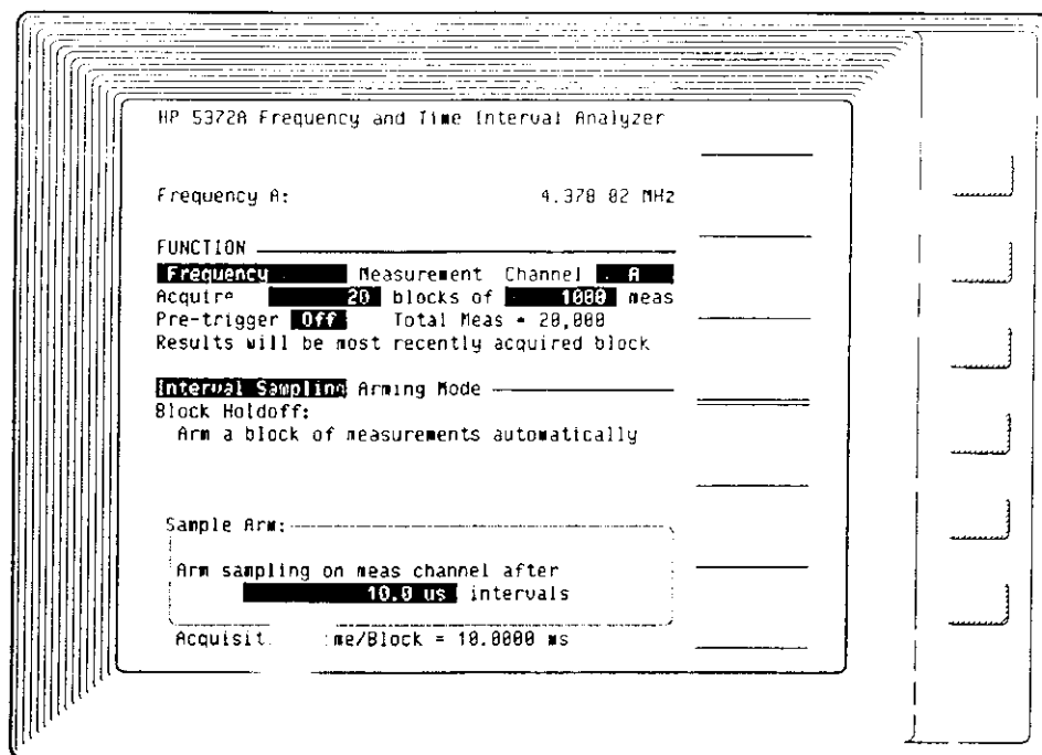
Figure 7-4. M Blocks — Measurements Do Not All Fit In Memory
