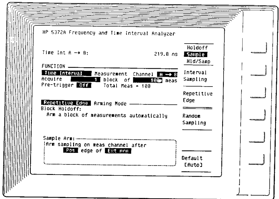
Figure 5-27. REPETITIVE EDGE Menu Screen
