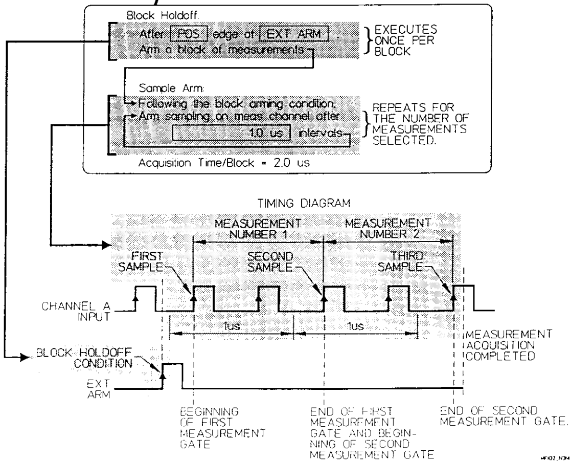
Figure 5-2. Group of Measurements
