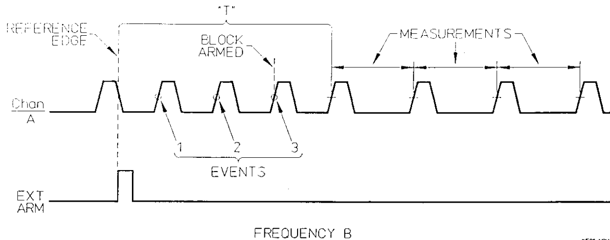
Figure 2-9. Frequency | Event Holdoff
