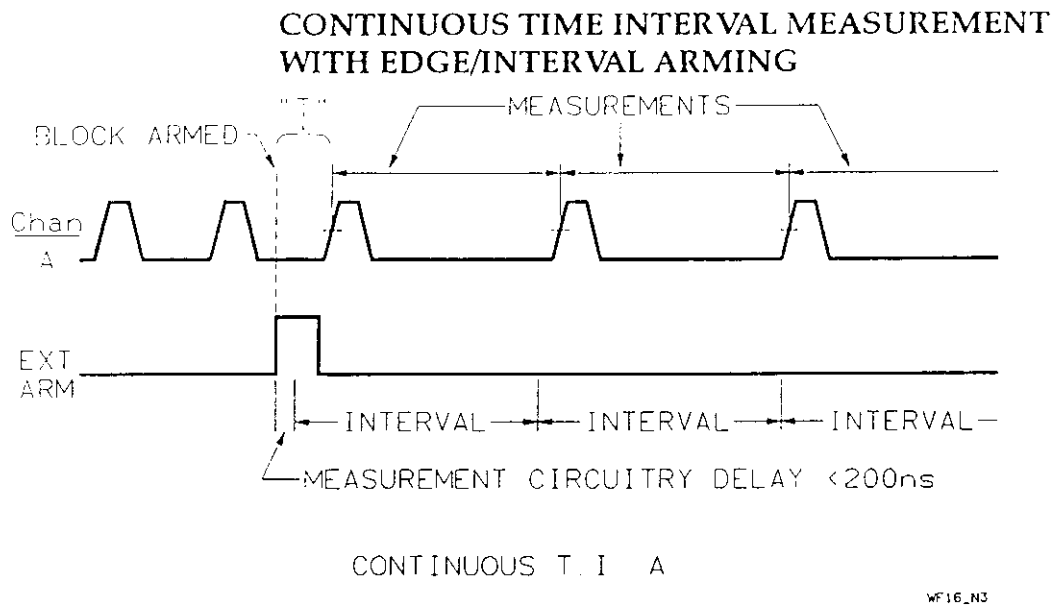
Figure 1-32. Continuous Time Interval | Edge/Interval
