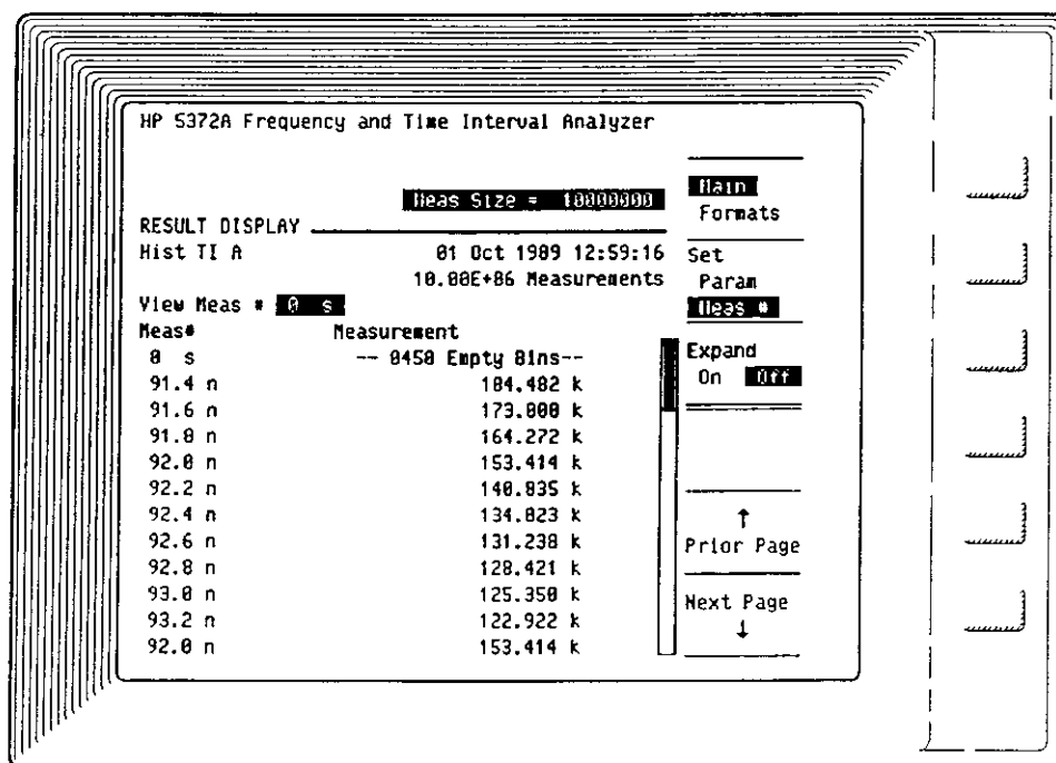
Figure 4-16. Numeric Results of Histogram Measurement, First Page
