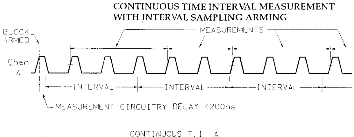
Figure 1-30. Continuous Time Interval | Interval Sampling
