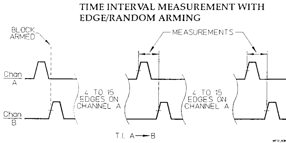
Figure 1-25. Time Interval | Edge/Random
