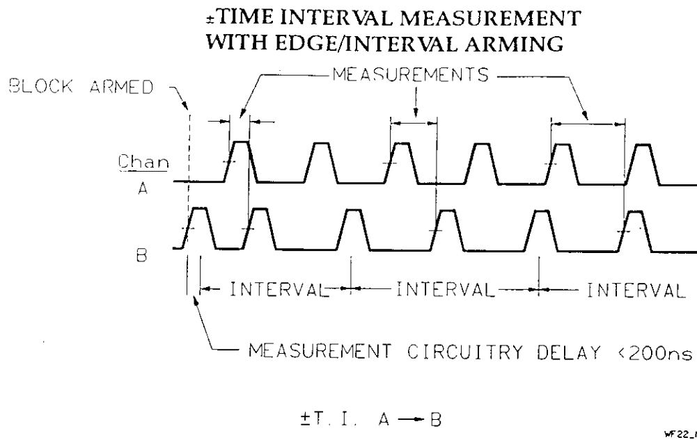
Figure 1-40. ±Time Interval | Edge/Interval
