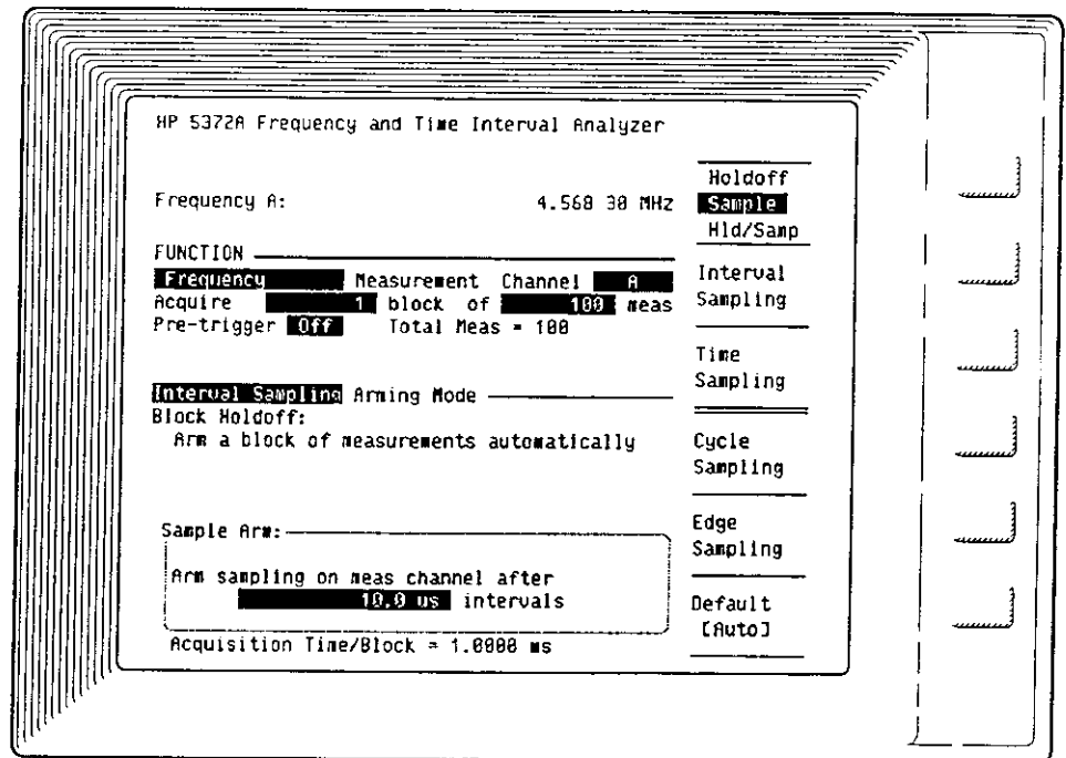
Figure 5-17. INTERVAL SAMPLING Menu Screen
