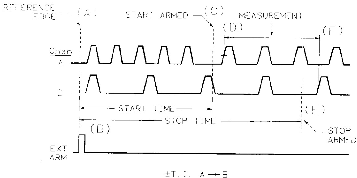
Figure 5-50. TIME/TIME Timing Diagram
