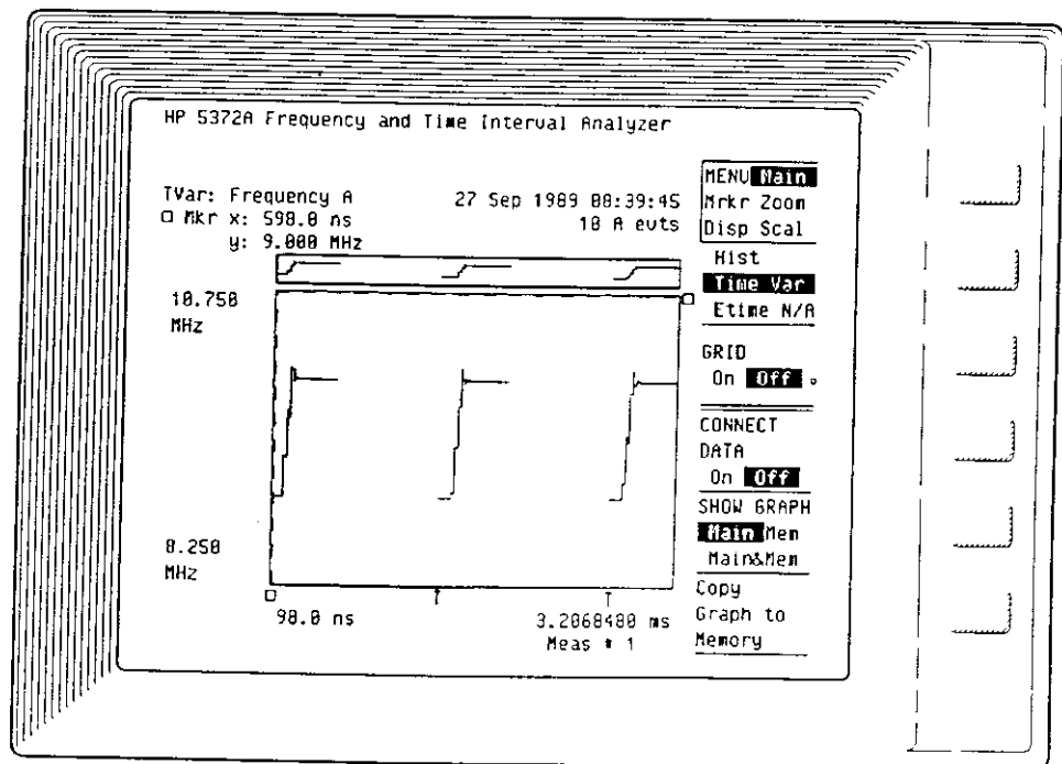
Figure 16-21. All Results Selected for Measurement Results
