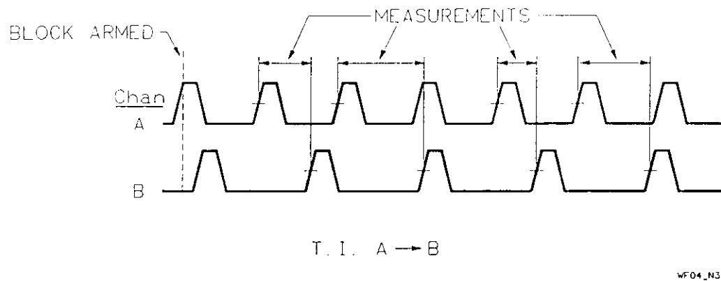
Figure 1-17. Time Interval | Automatic
