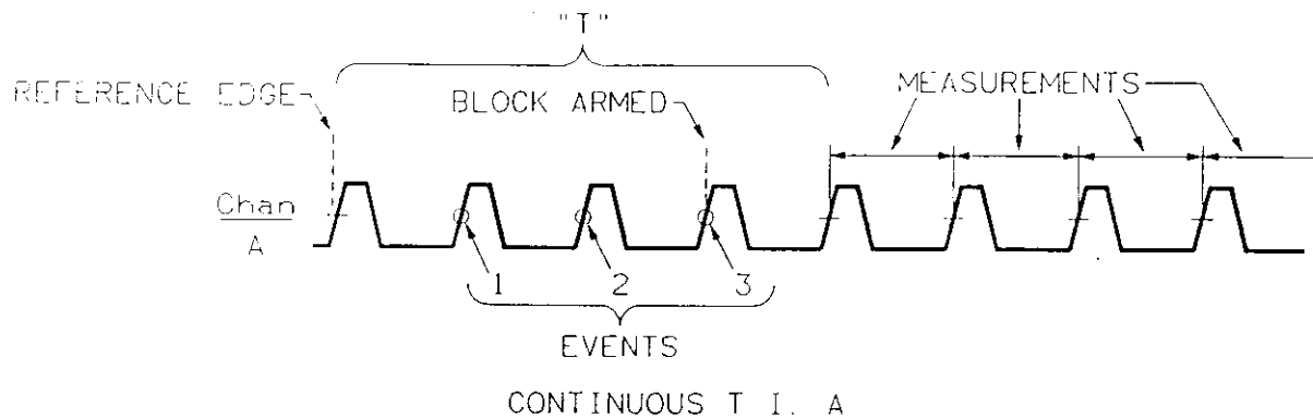
Figure 1-29. Continuous Time Interval | Event Holdoff
