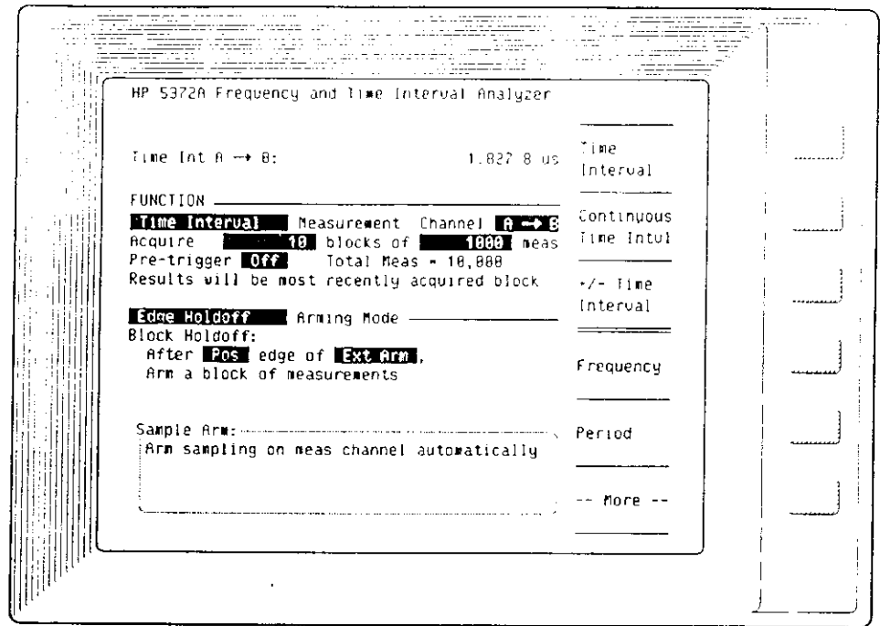
Figure 16-11. UPDATE While or After Selection is Available
