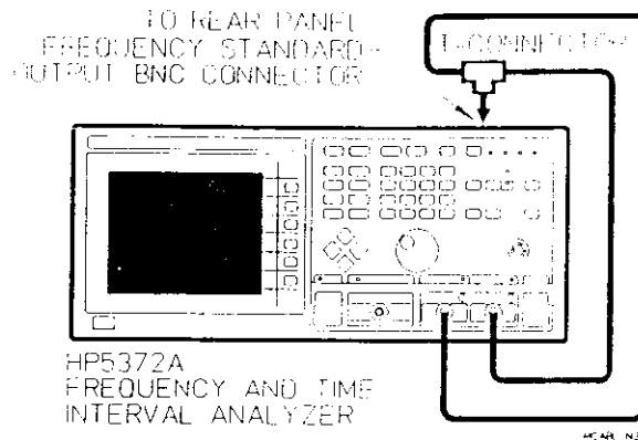
Figure 17-1. HP 5372A Operation Verification Setup
