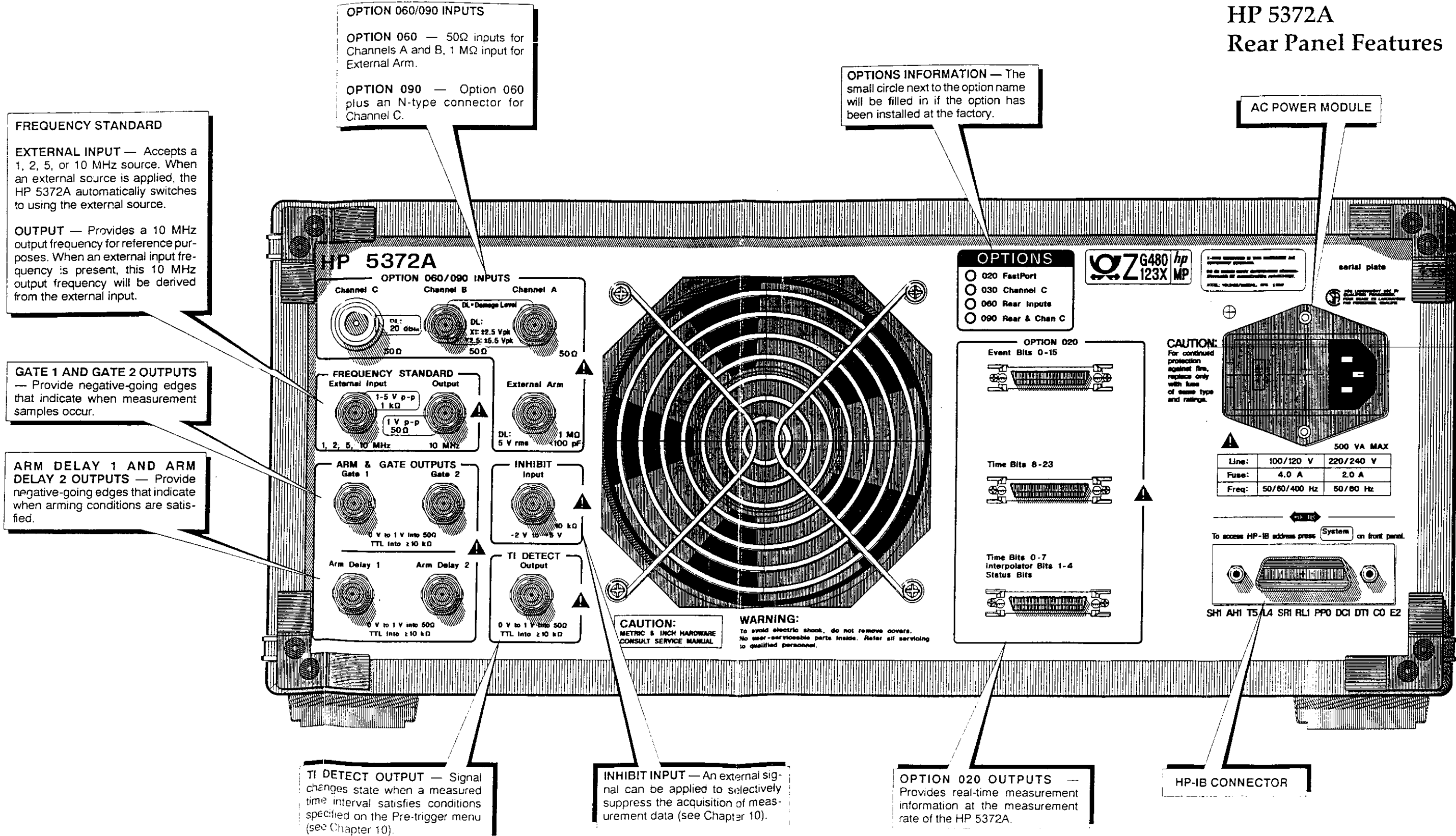
Figure 6-2. Rear Panel Features
