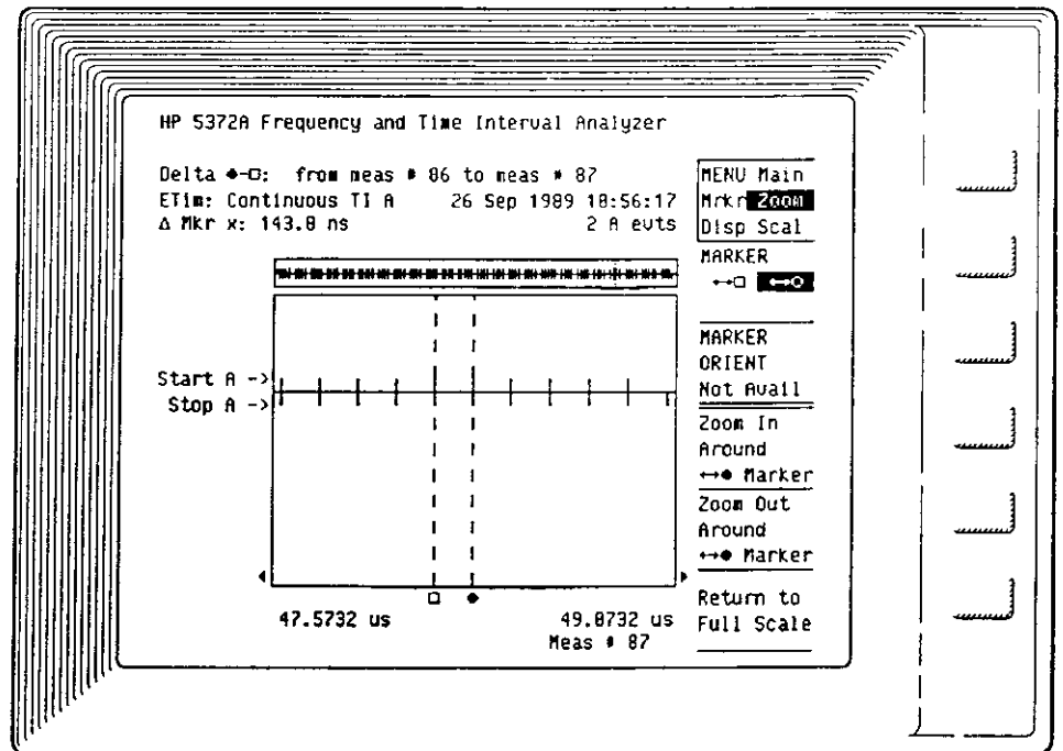
Figure 1-16. Event Timing Graph of CTI
