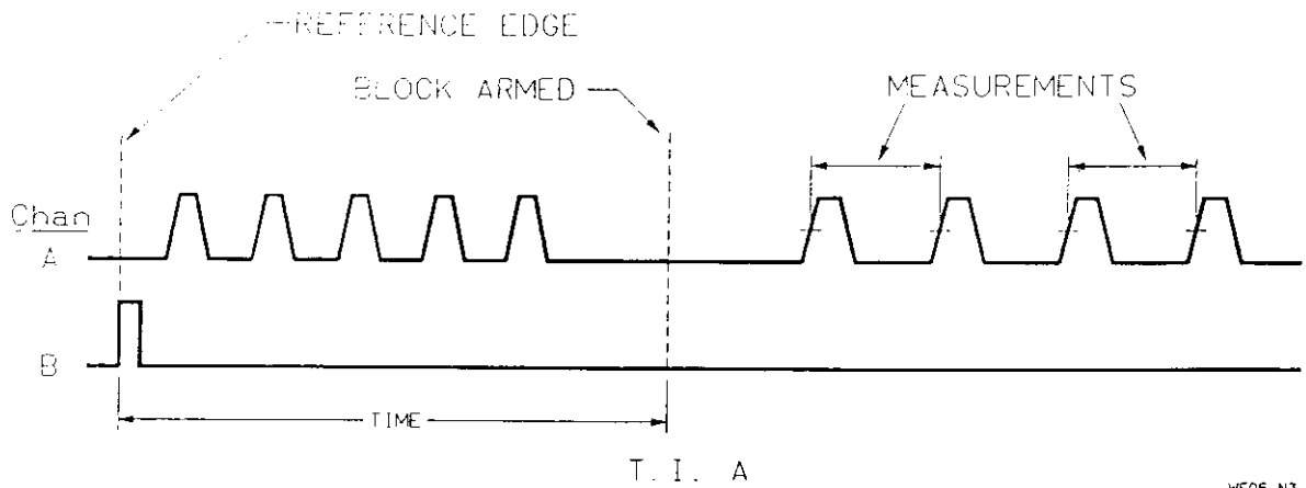
Figure 1-19. Time Interval | Time Holdoff
