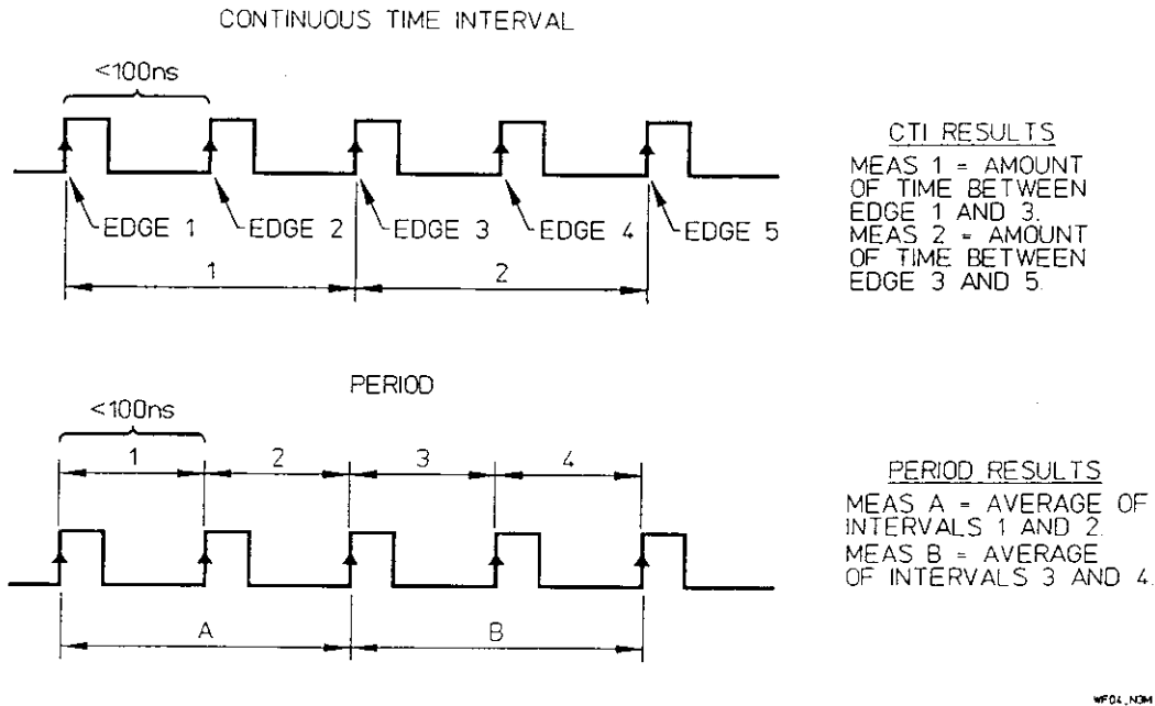
Figure 1-5. Continuous TI vs. Period
