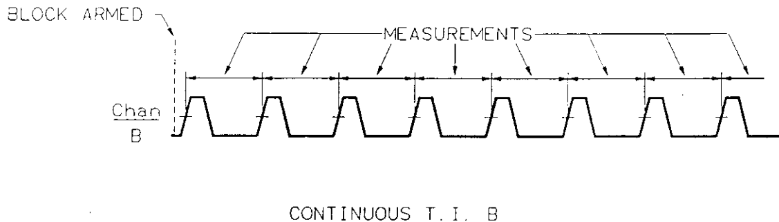
Figure 1-26. Continuous Time Interval | Automatic
