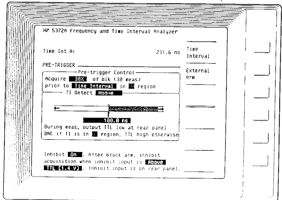
Figure 10-1. Pre-trigger Menu Screen
