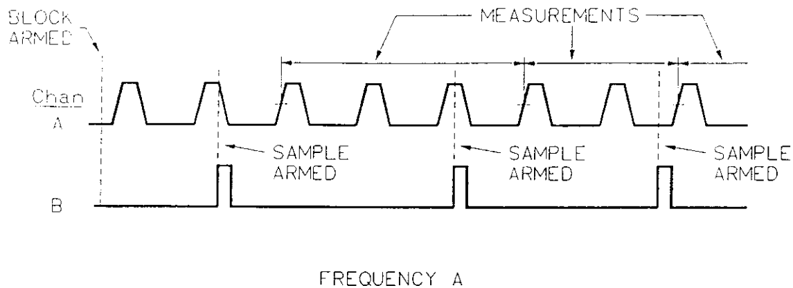
Figure 2-13. Frequency | Edge Sampling
